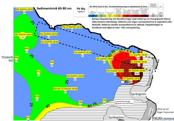
Figur 4: Bly 60-80 cm.
