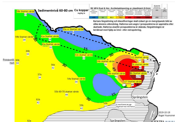
Figur 8: Koppar 60-80 cm.
