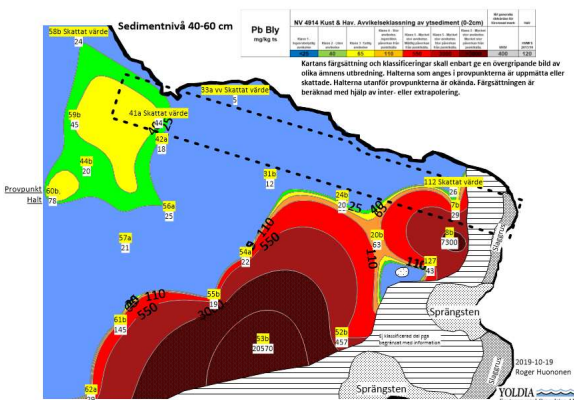
Figur 3: Bly 40-60 cm.
