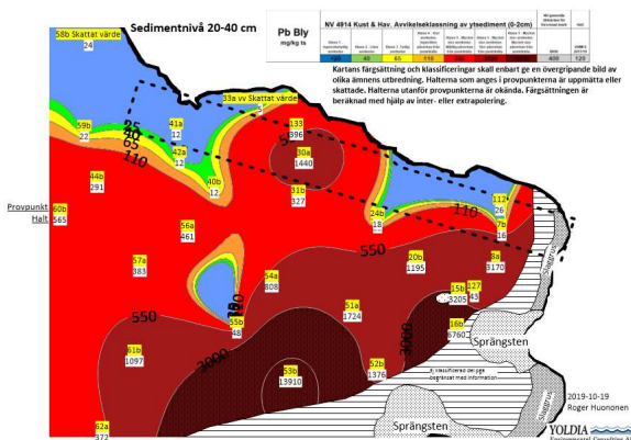
Figur 2: Bly 20-40 cm.
